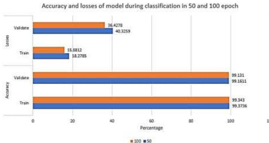
Figure 3: Accuracy and losses of model during classification in 50 and 100 epochs
