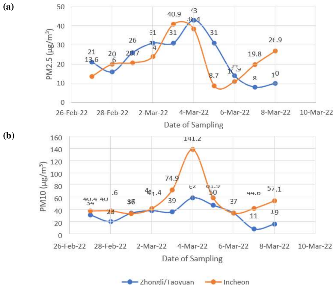
Figure 4. The Comparison of (a) PM_{2.5} & (b) PM_{10} between Zhongli/Taoyuan vs Incheon
