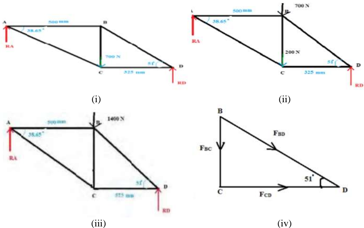
Figure 1. (i) Static start-up, (ii) Steady pedalling (iii) Vertical loading, and (iv) Rear wheel braking
