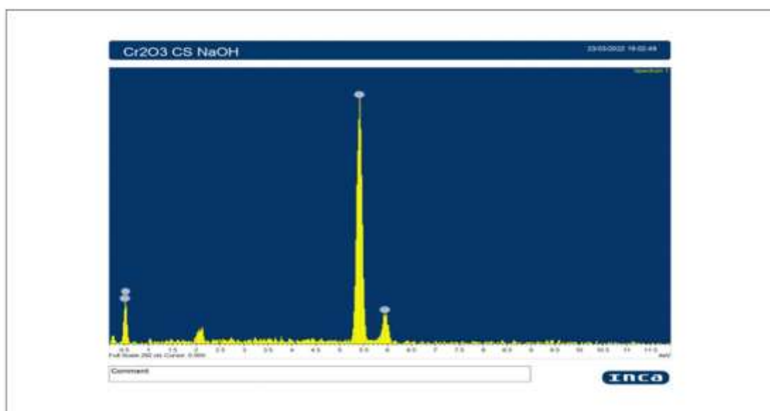
Figure 3. EDX spectrum of chemically synthesized \text{Cr}_2\text{O}_3 NPs
