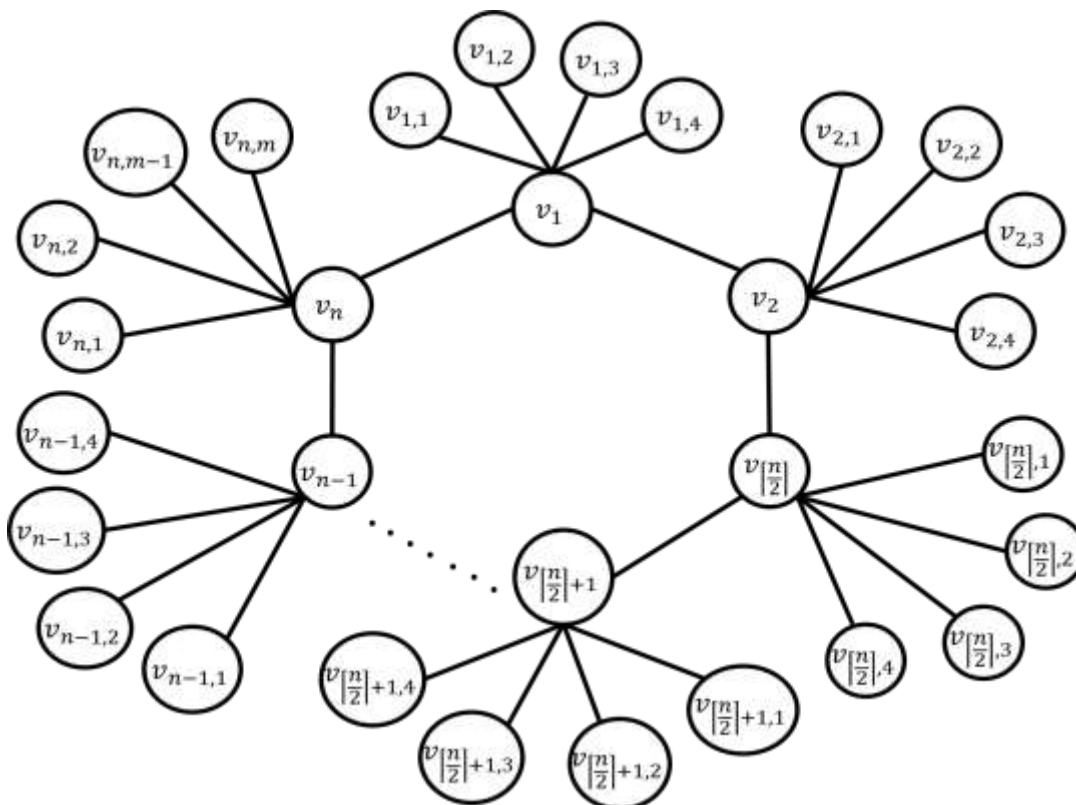
Figure 1. Hairy cycle graph C_m^n with m = 4
