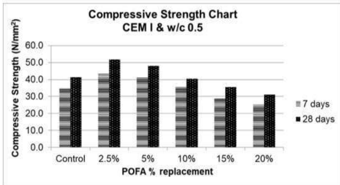
Figure 1. Compressive Strength of Concrete after adding POFA (Ash, 2018)
