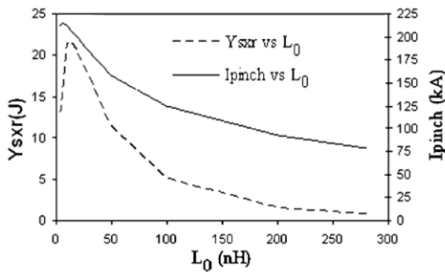
Fig. 10 The X-ray yield and I_{pinch} (computed) versus L_0 (280–3 nH) at 15 kV, 2.8 Torr of Neon
