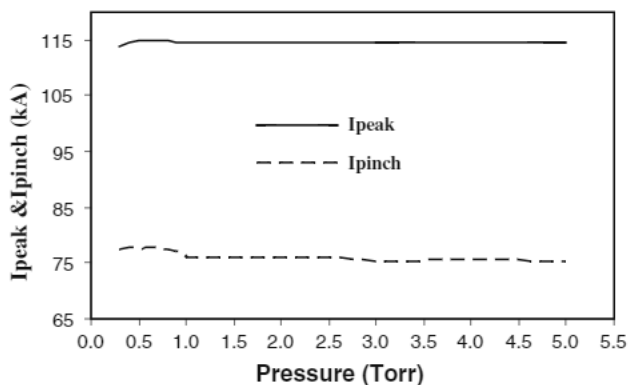
Fig. 8 Effect on currents I_{peak} and I_{pinch} as p_0 is increased from 0.3 to 5 Torr
