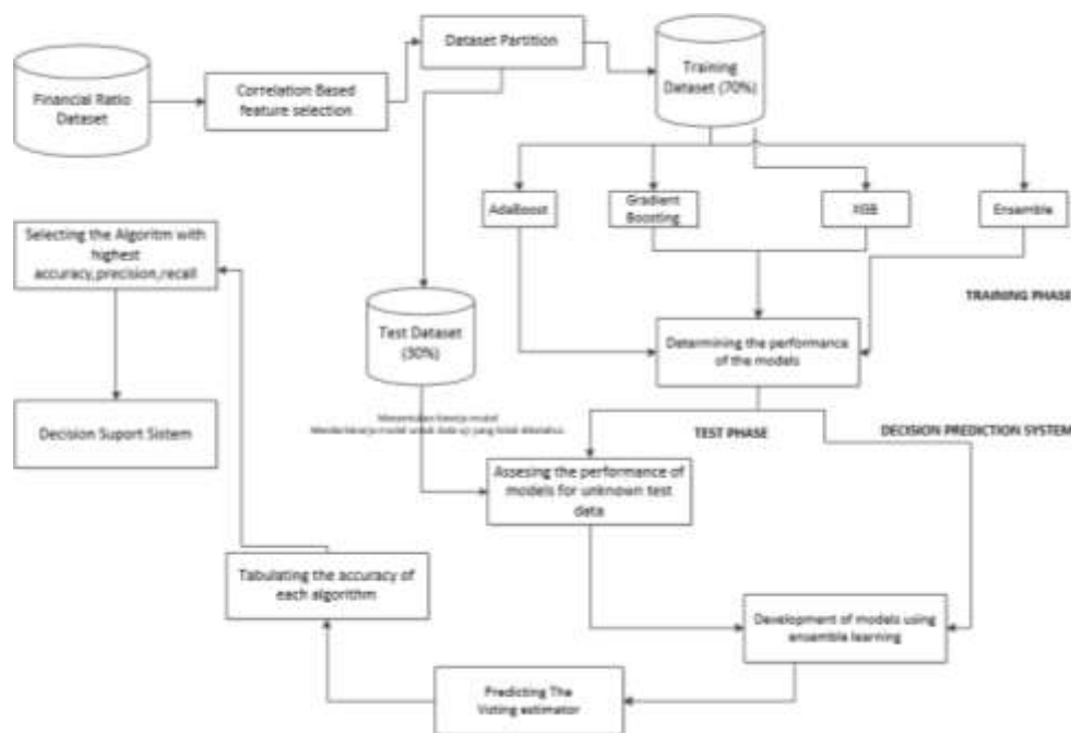
Figure 1. Boosting Clasifier Method
